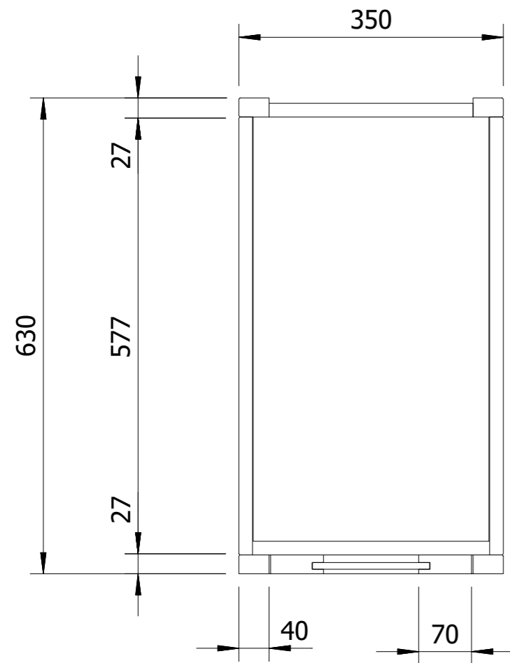
SECTION B-B
