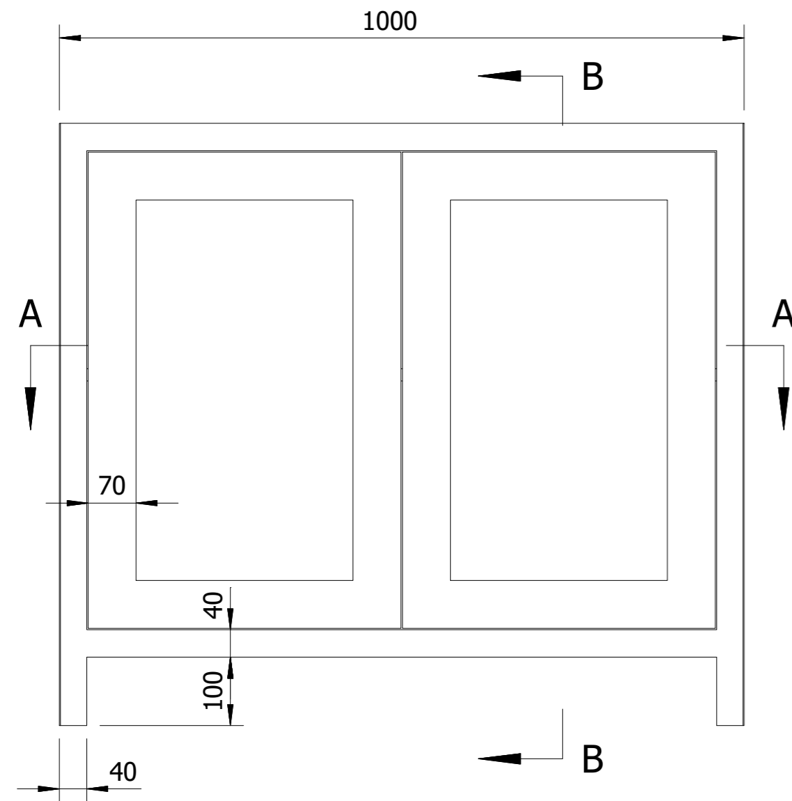
FRONT ELEVATION
