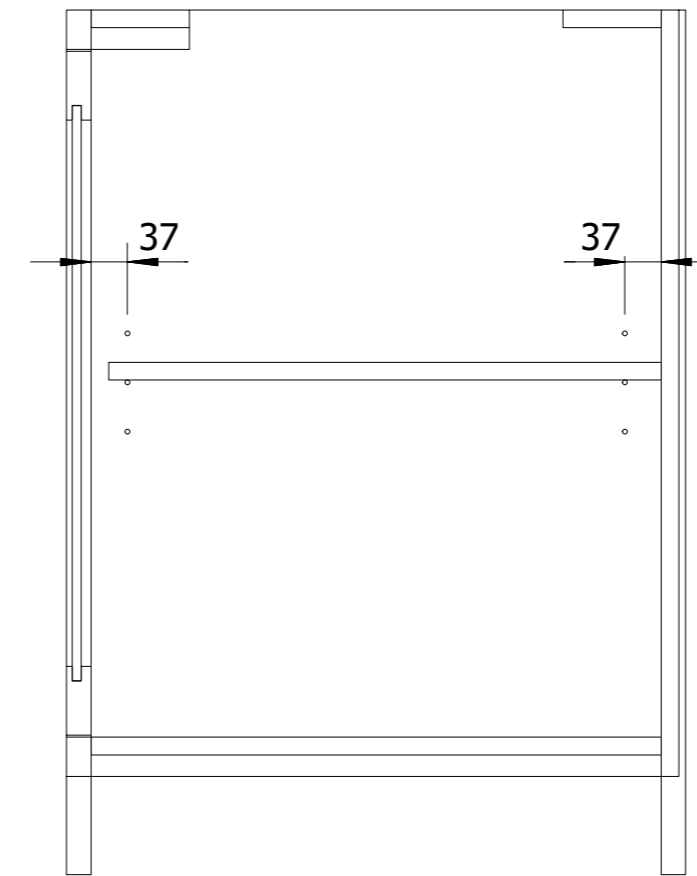
SECTION B-B
