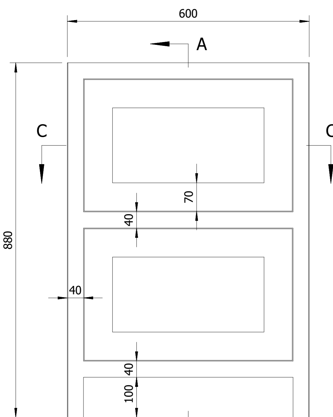
FRONT ELEVATION
