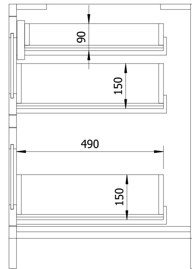
SECTION B-B
