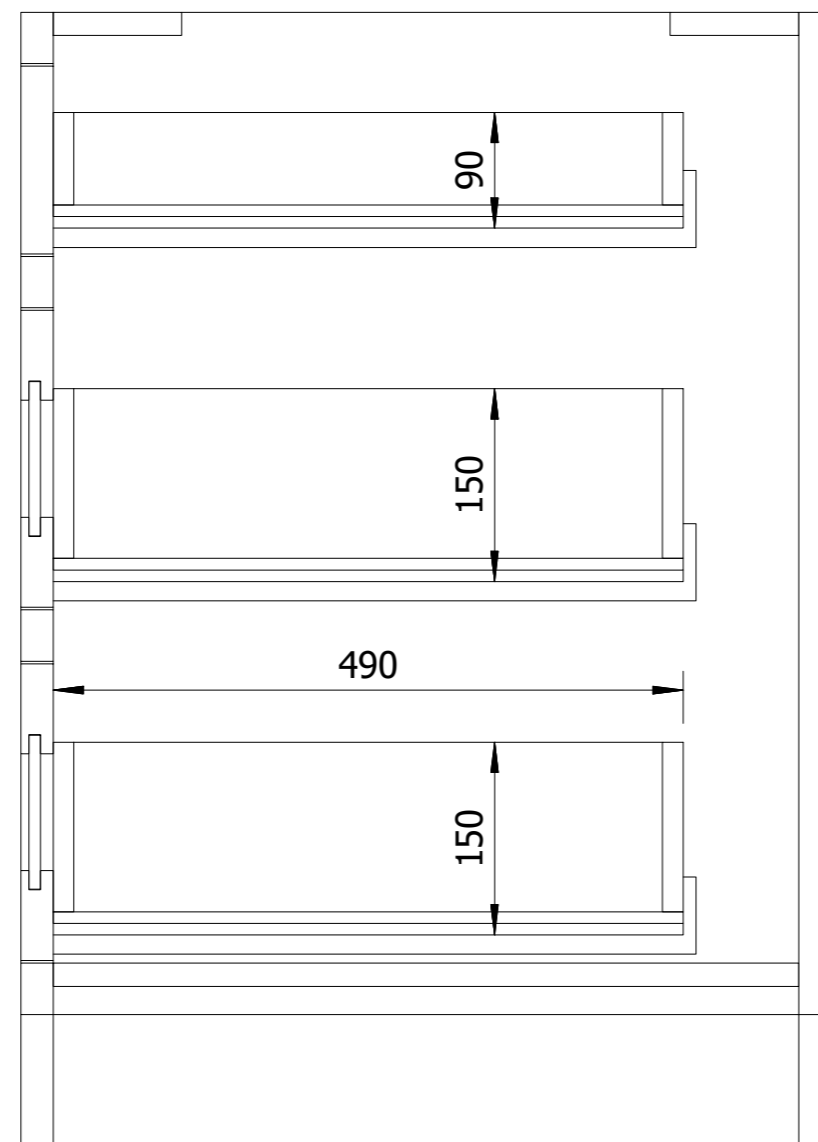
SECTION B-B
