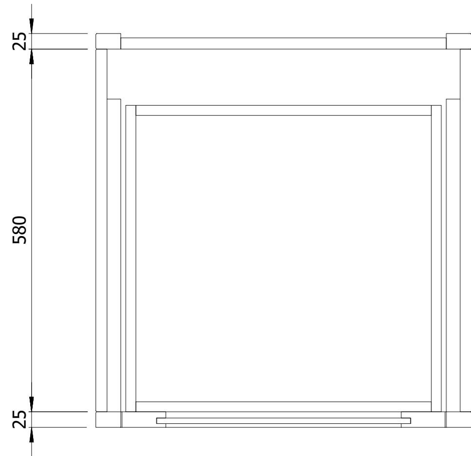
SECTION C-C
