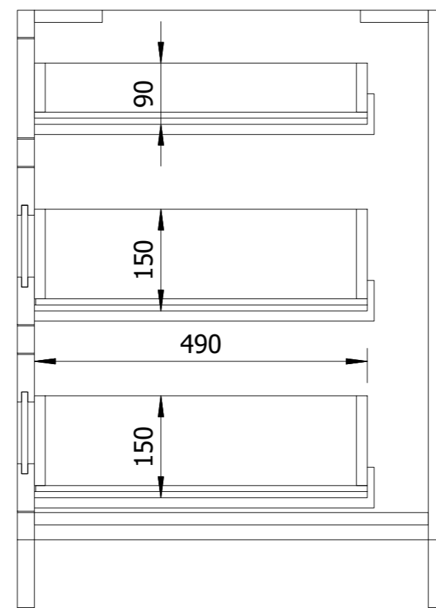
SECTION B-B
