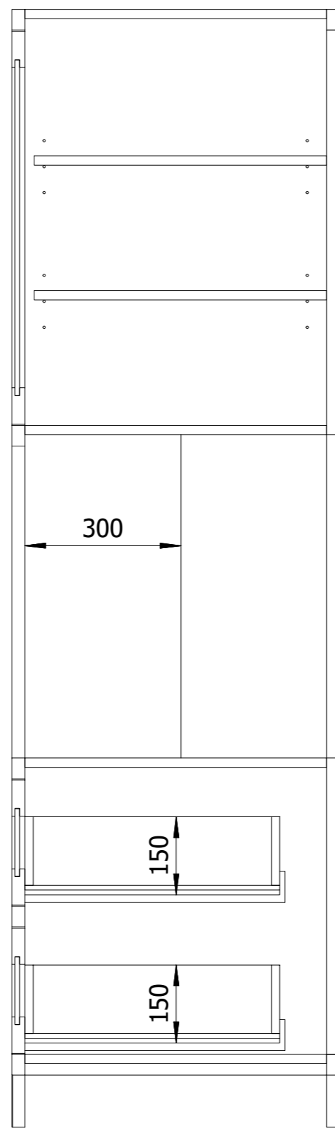
SECTION C-C
