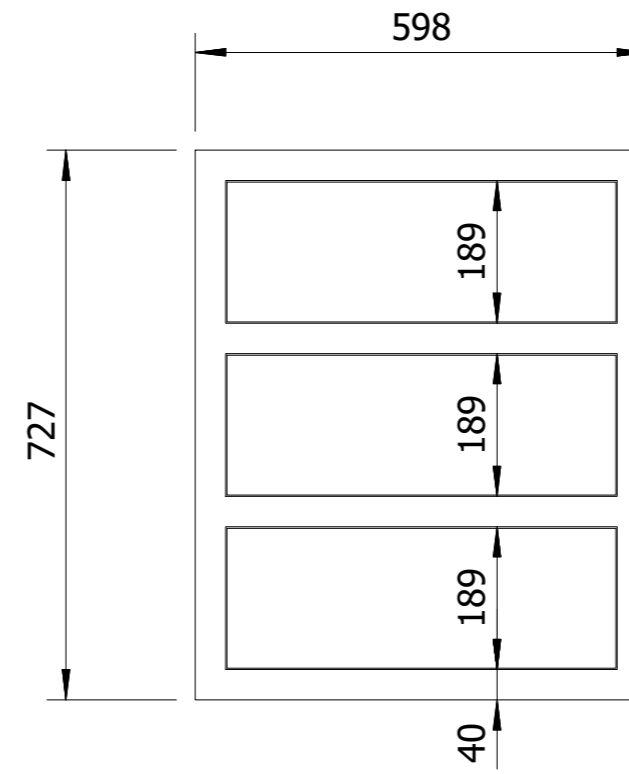
INTERNAL DRAWERS
