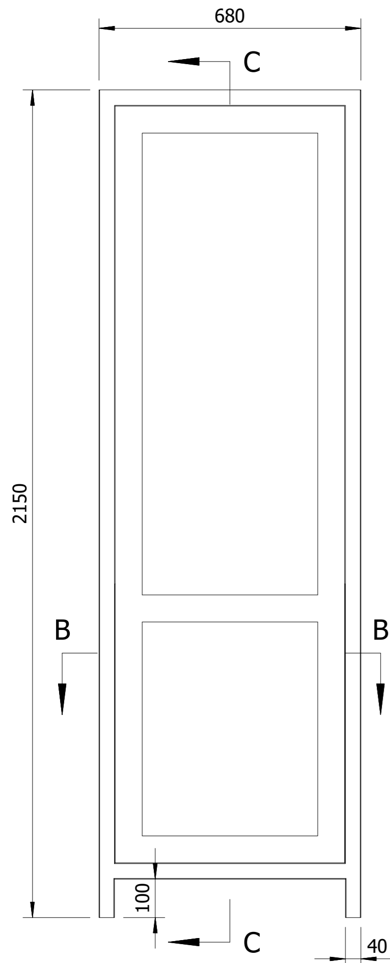
FRONT ELEVATION
