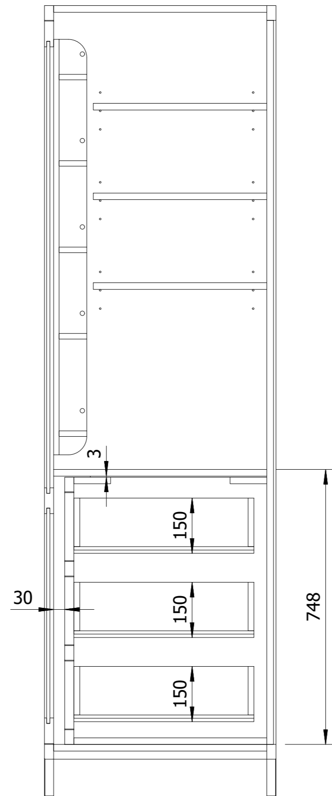
SECTION C-C
