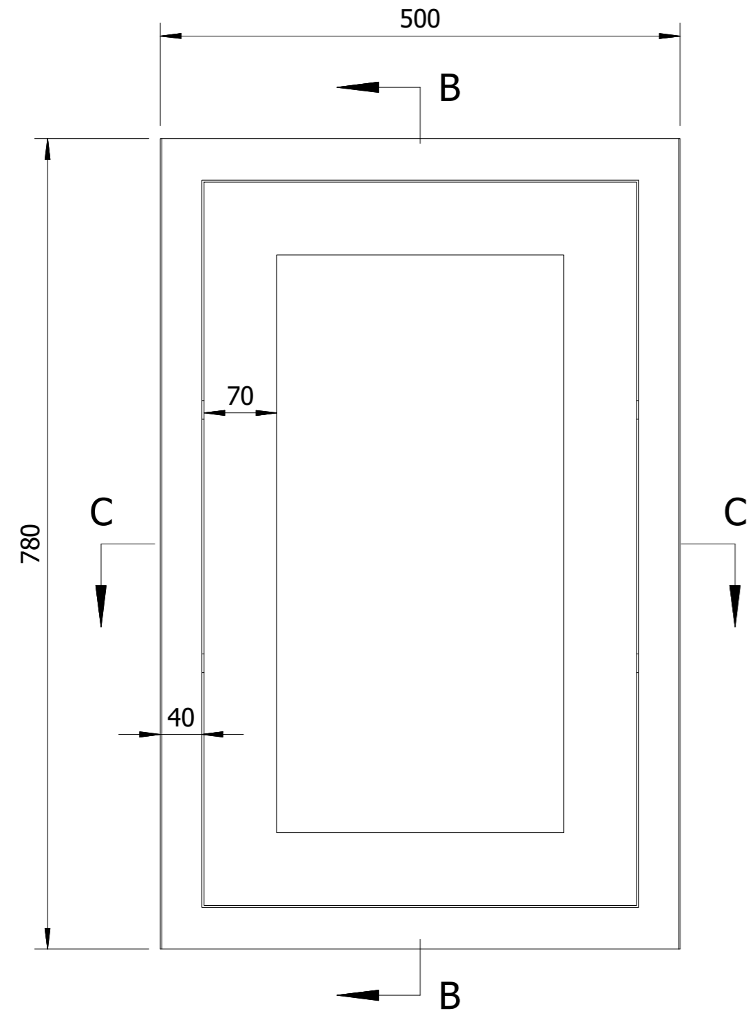
FRONT ELEVATION
