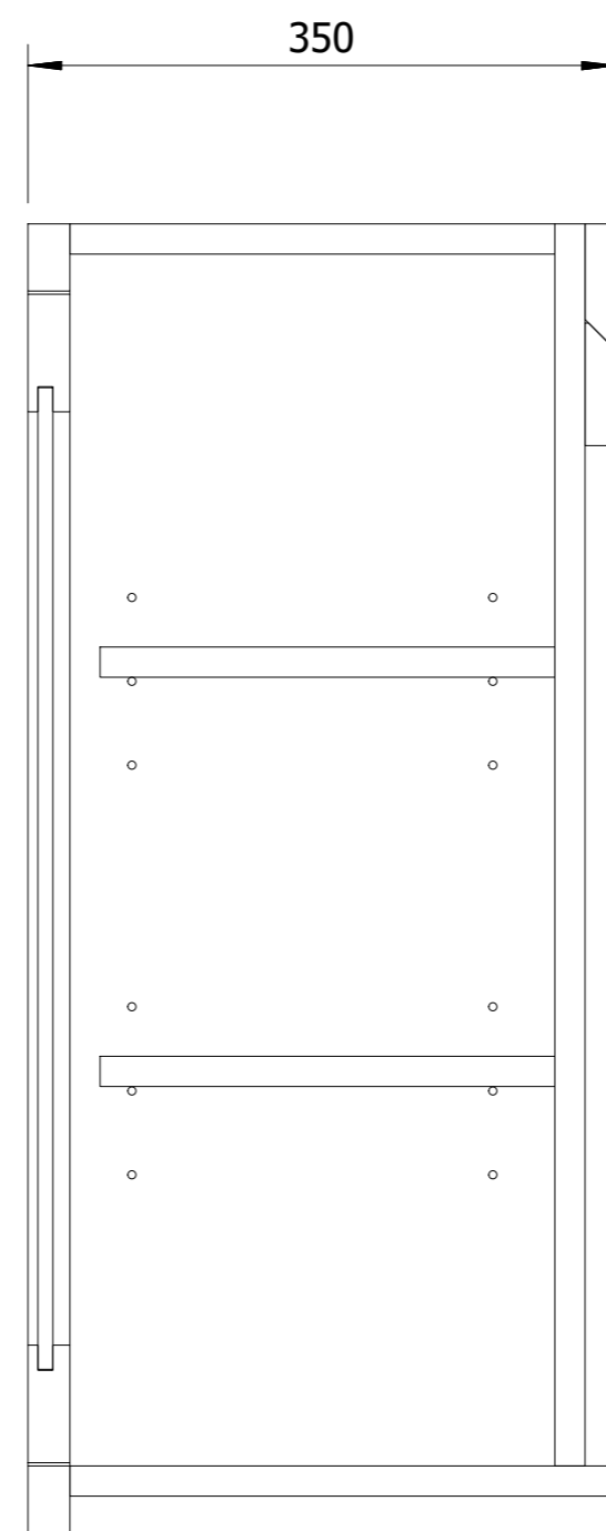
SECTION B-B
