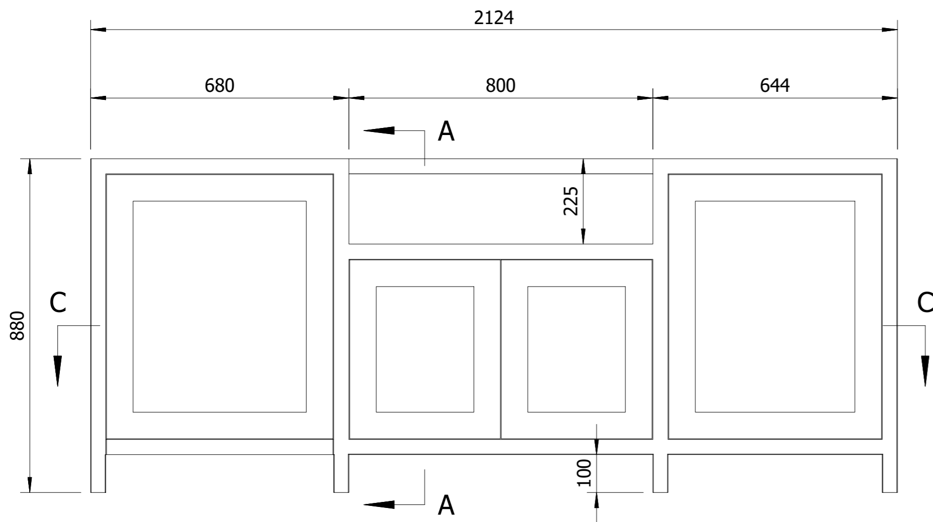
FRONT ELEVATION
