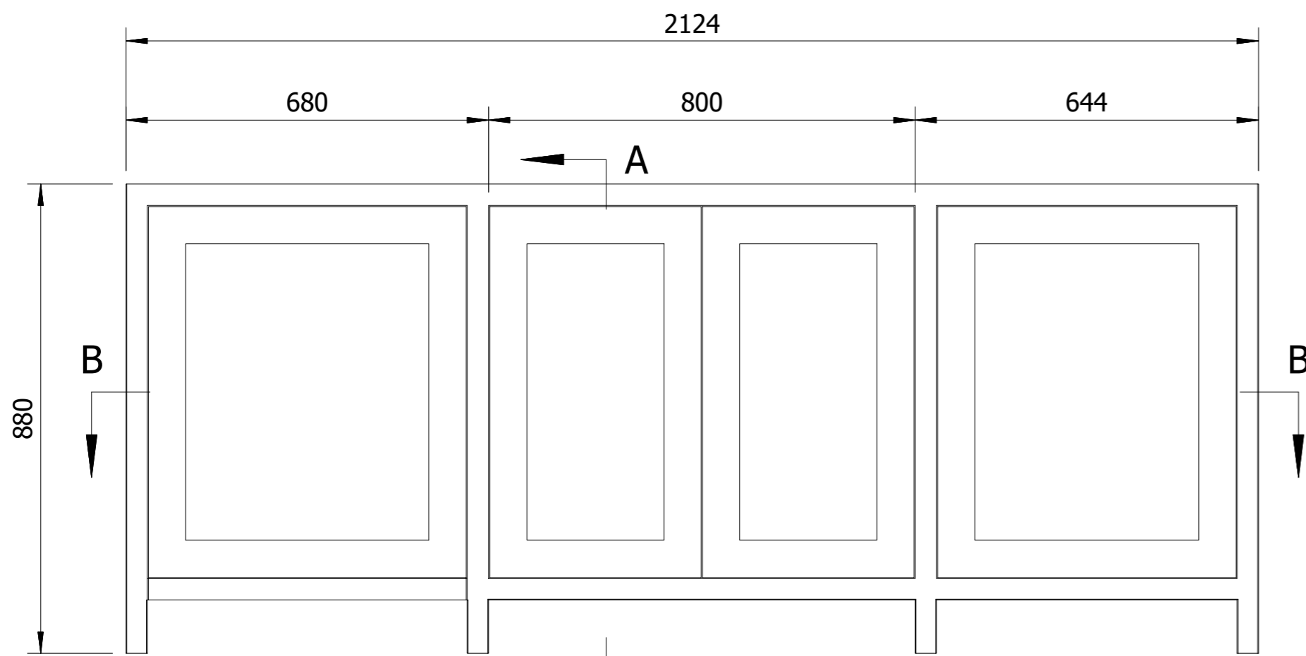
FRONT ELEVATION
