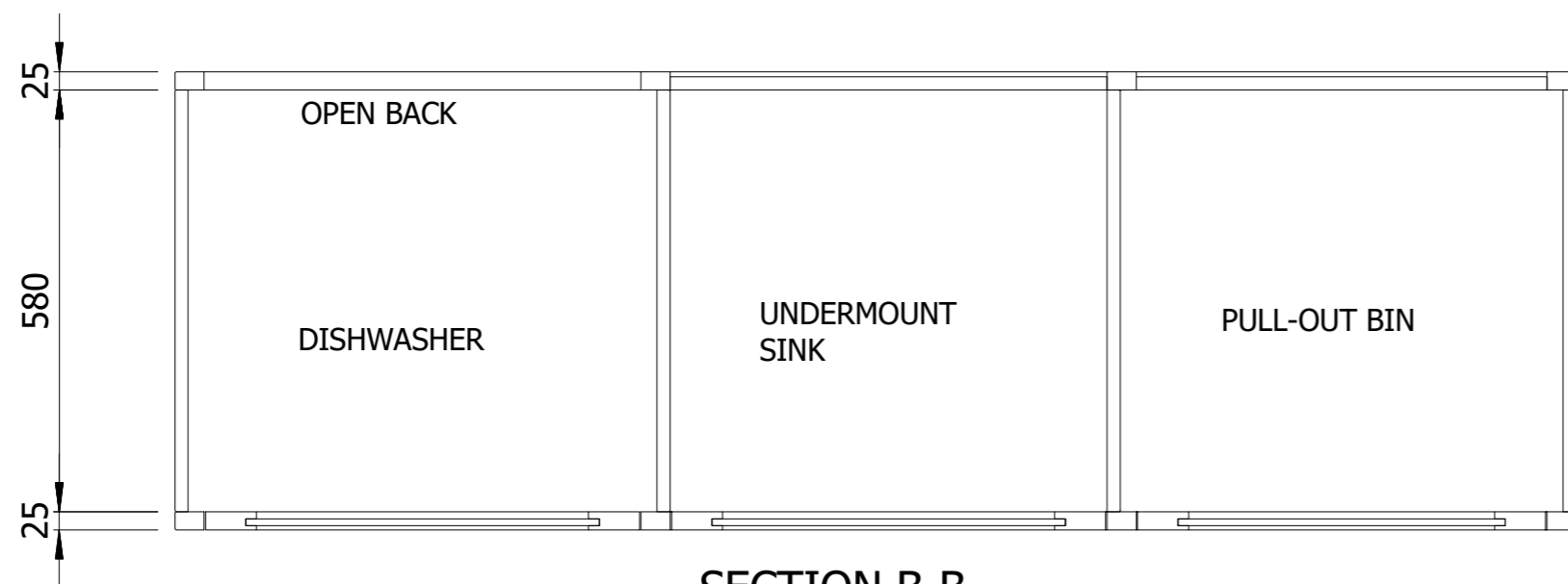
SECTION B-B
