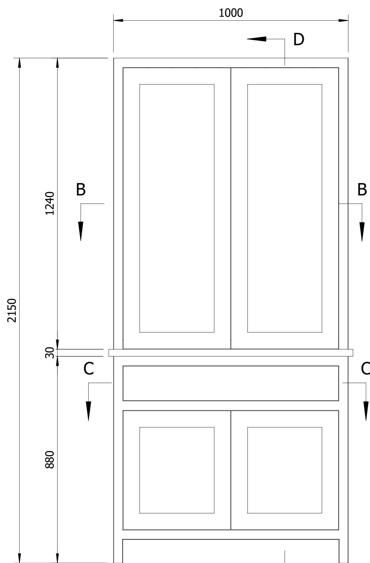
FRONT ELEVATION
