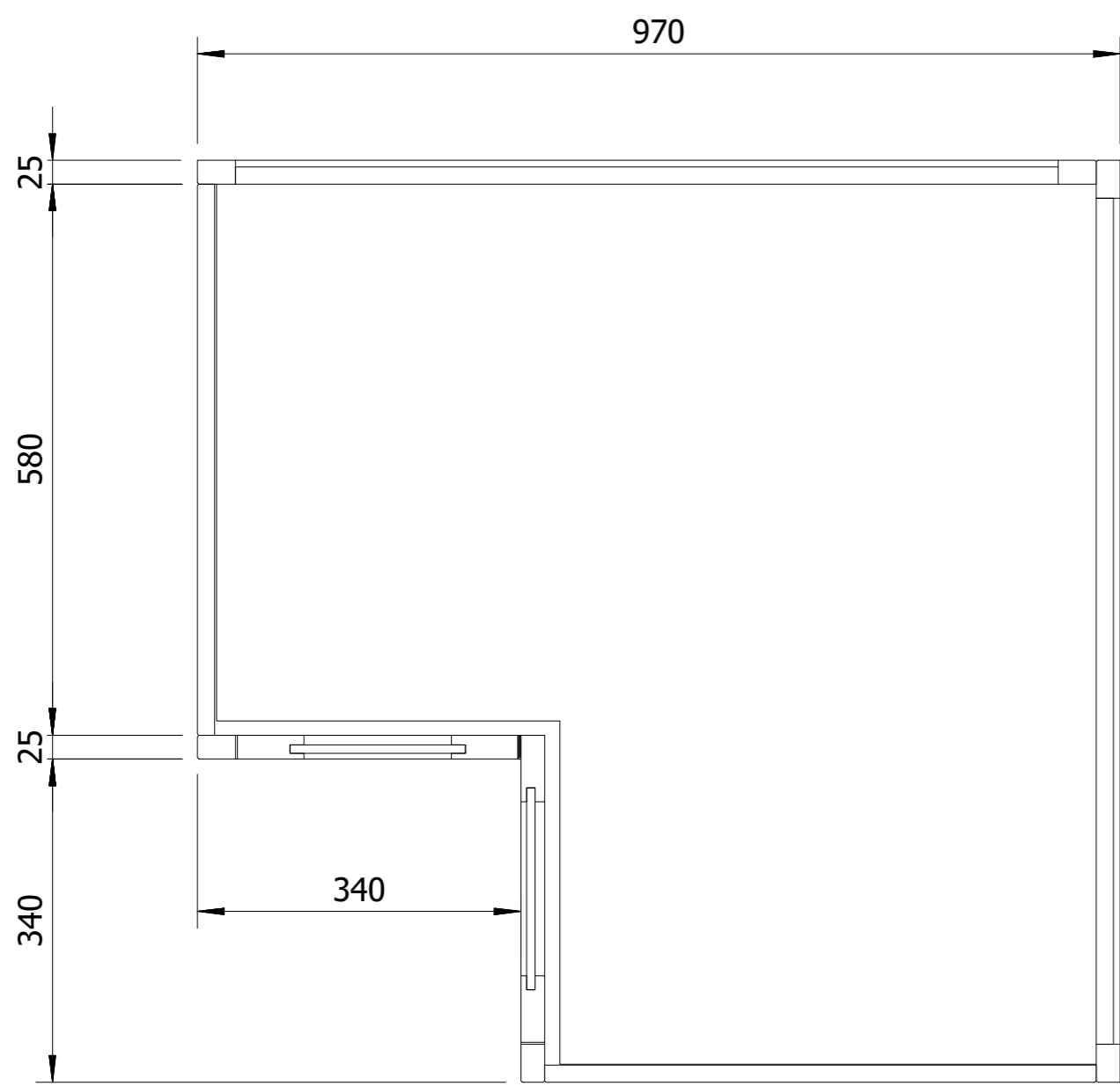
SECTION C-C
